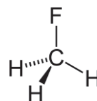
Fluoromethane
